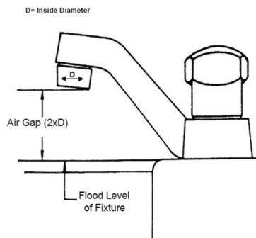
Air Gap And Effective Opening
